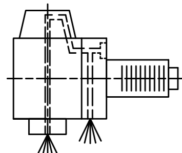
Innen- und Aussenkuehlung / Inside and outside coolant supply Kuehlmittefiltration-50 \mu / coolant filtration-50 \mu
