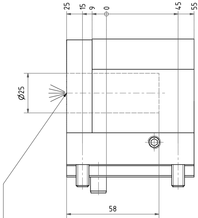
Hydrodehnfutter / hydraulic chuck NBC-25/32-50
