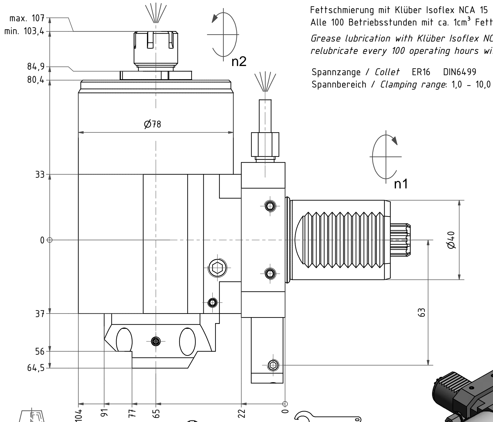
Hakenschlüssel mit Nase Hook wrench with nose end DIN1810 A 36x38
