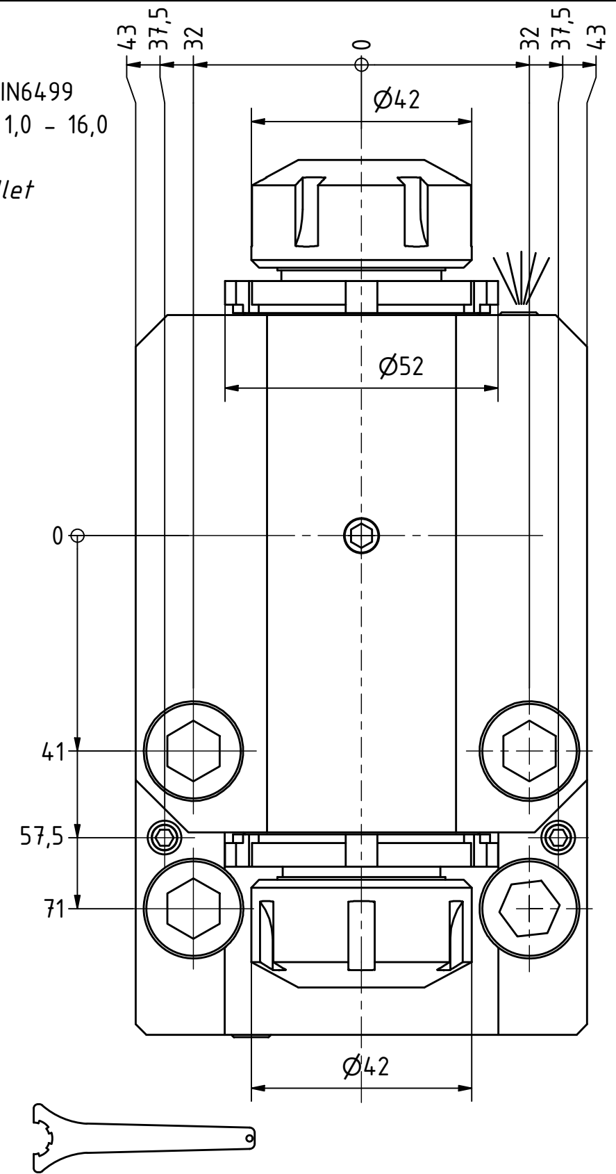
Spannzangenschlüssel Clamping wrench 225
