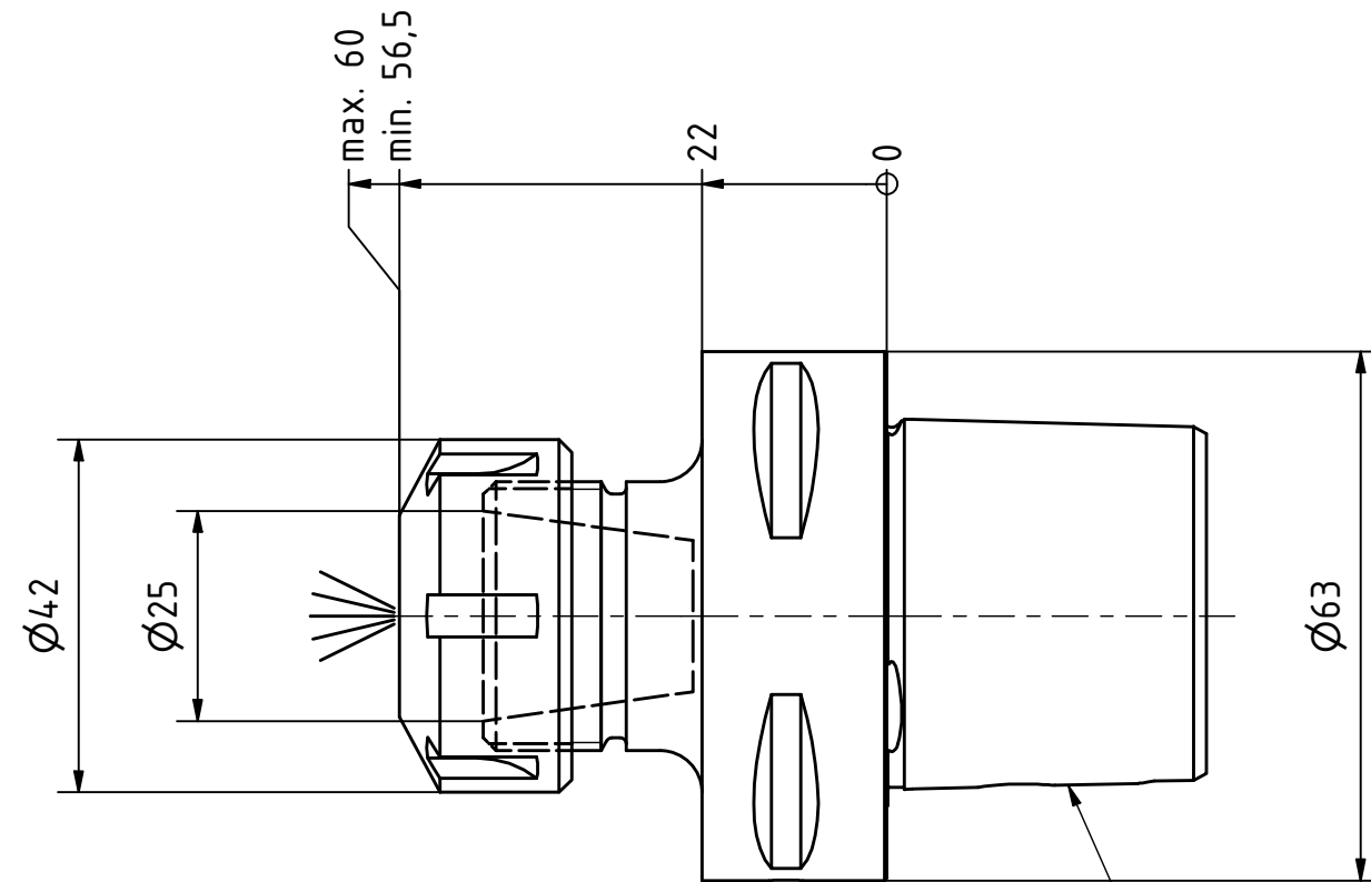
Polygon ISO 26623 PSC 63
