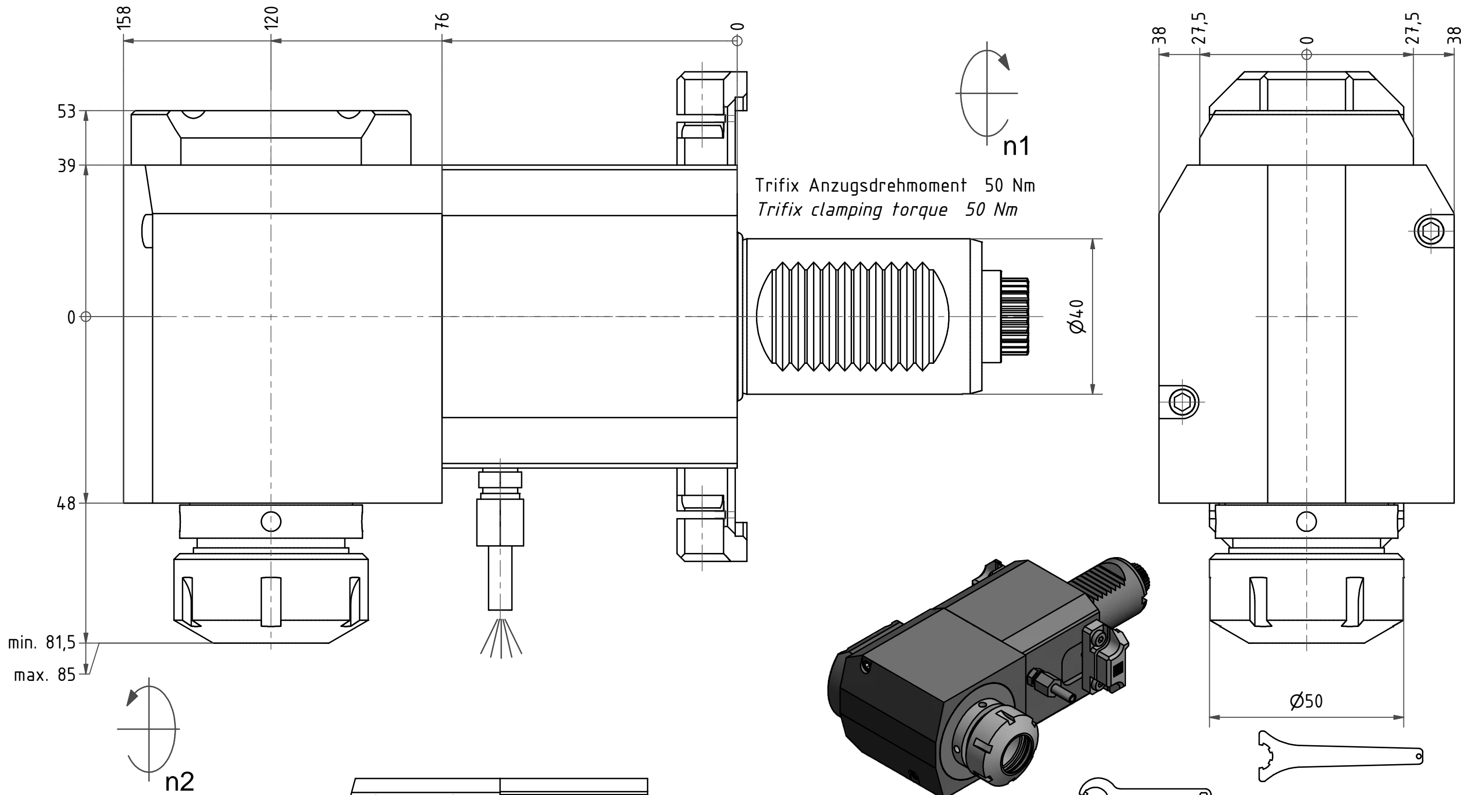
Spannzangenschlüssel Clamping wrench 232
