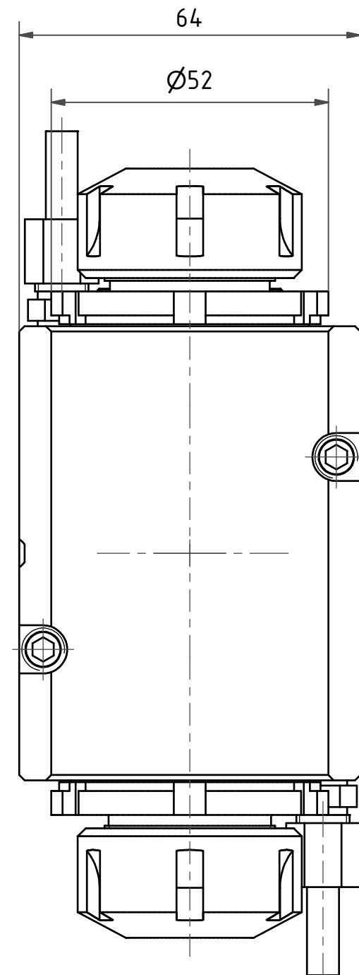
Hakenschlüssel mit Nase Hook wrench with nose end DIN1810 A 52x55 Spannzangenschlüssel Clamping wrench 225
