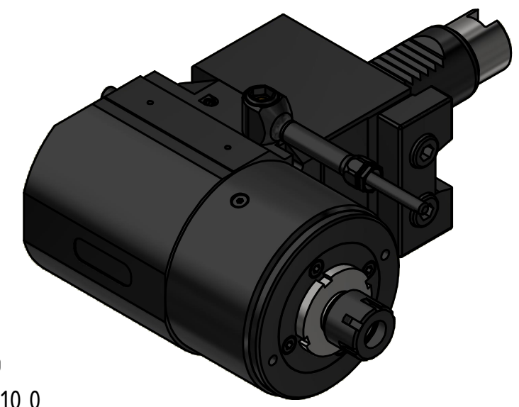
Hakenschlüssel mit Nase Hook wrench with nose end DIN1810 A 36x38 Spannzangenschlüssel Clamping wrench 216 M
